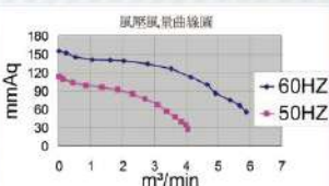
CX-1/2 0.4KW
