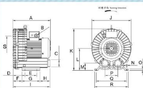
LG-006 1/8HP
